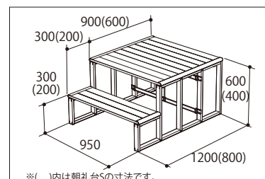
AL-CL (朝礼台L)
